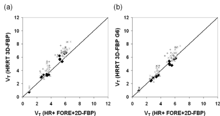
Fig 1. Correlation between parametric human [ 11 C]flumazenil Logan V_T obtained with various HRRT reconstruction methods against corresponding Logan V_T obtained with HR+ 2D-FBP+FORE: (a) 3D-FBP, (b) 3D-FBP smoothed with 6 mm full width at half maximum Gaussian kernel.
